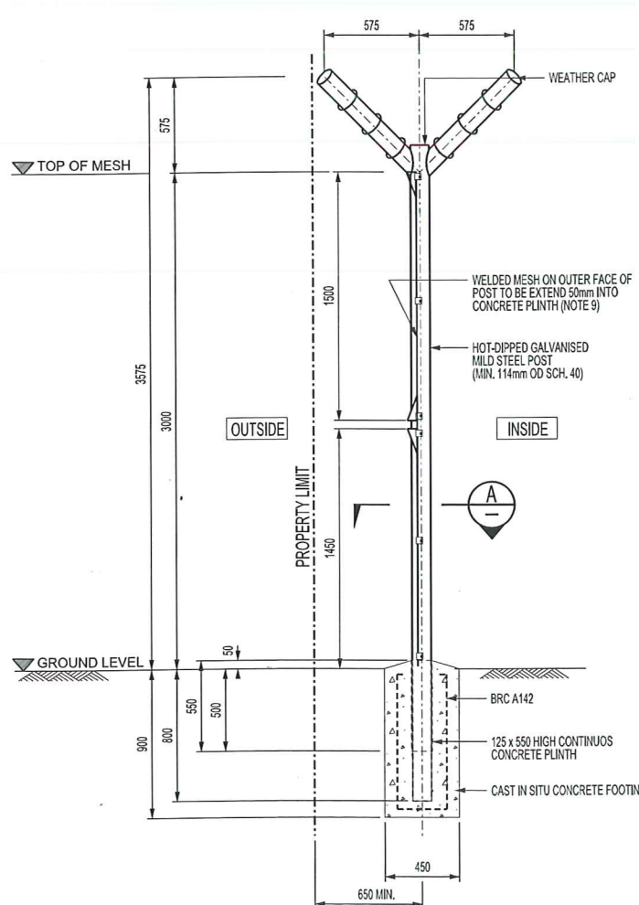
TUBULAR POSTS PERIMETER SECURITY FENCING SCALE 1:20
