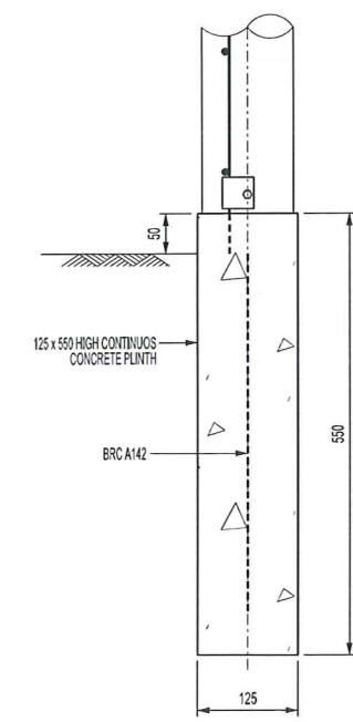
SECTION B SCALE 1:5
