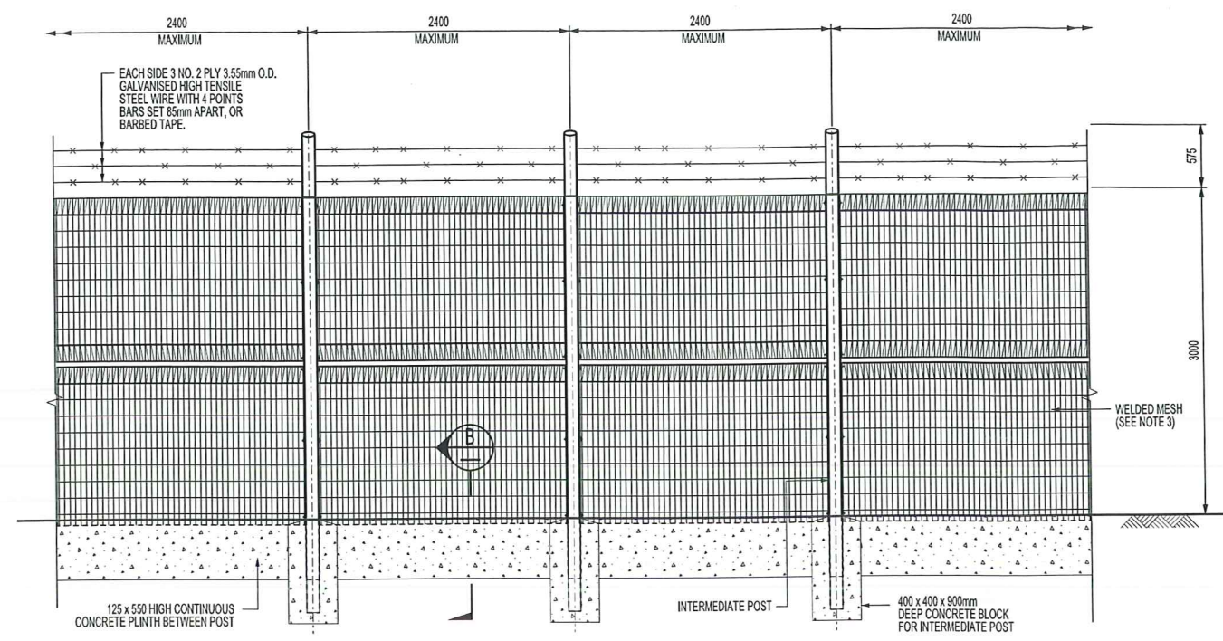
ELEVATION PERIMETER SECURITY FENCING DETAILS SCALE 1:30
