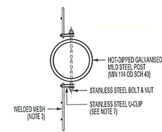
SECTION A SCALE 1:5
